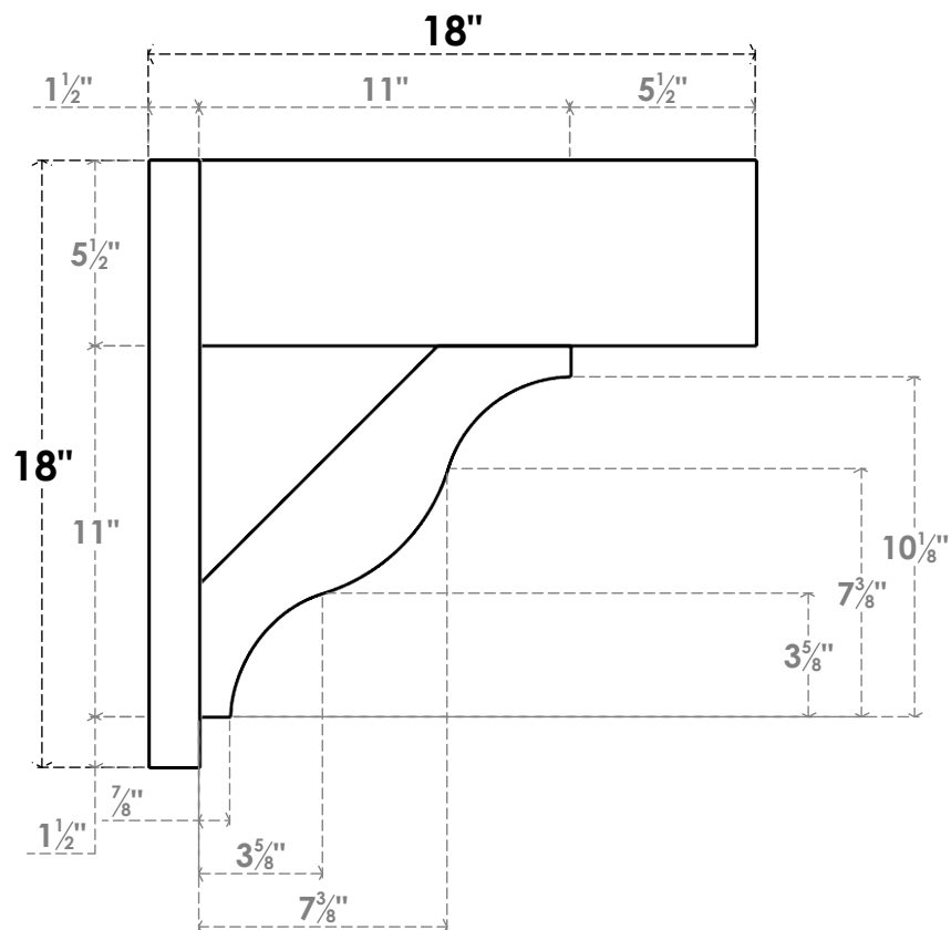
SIDE PROFILE
